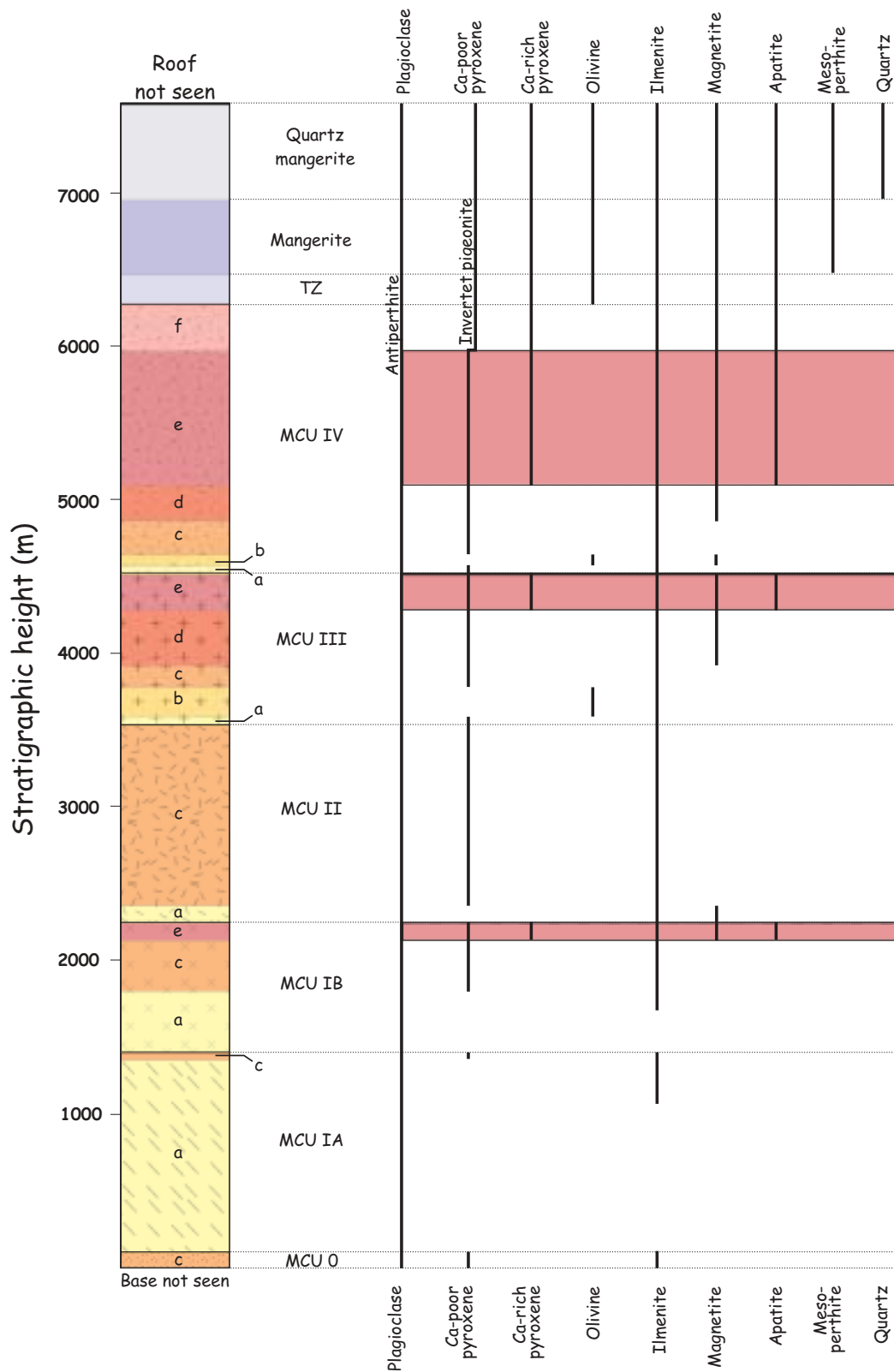
Fig. 2. Cumulate stratigraphy in the Bjerkreim-lobe of the Bjerkreim-Sokndal Layered Intrusion. The layered series is made up by 6 megacyclic units (MCU's) subdivided into a sequence of zones (a-f), defined by the presence or absence of certain index minerals. Three apatite-bearing sequences are found in the Bjerkreim-lobe (expanded red intervals): MCU IBe, MCU IIIe and MCU IVe-f.
