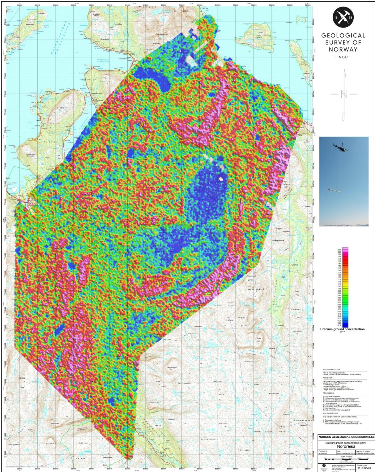
Figure 13: Uranium ground concentration
