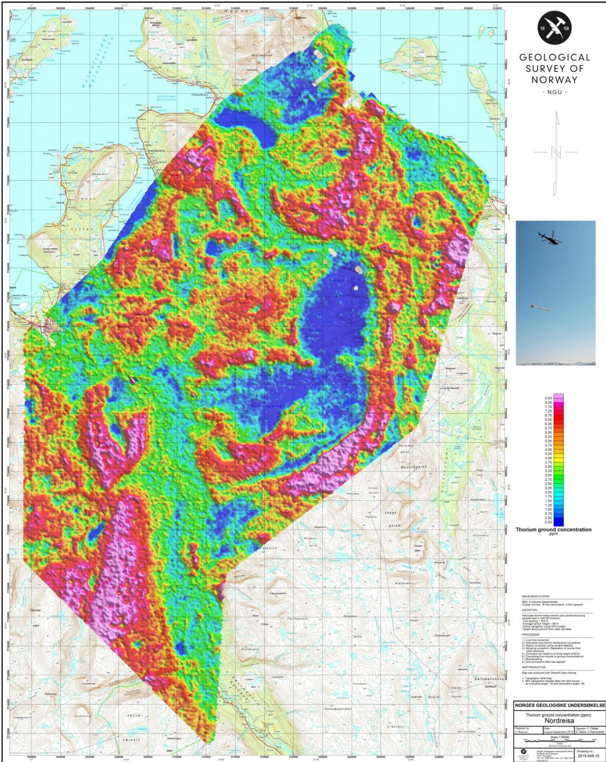
Figure 14: Thorium ground concentration
