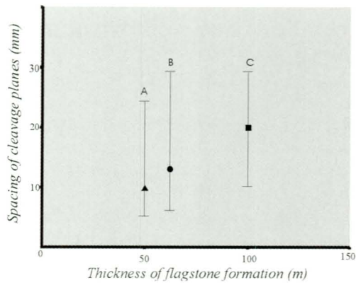
Fig. 4. Average spacing of cleavage (slab thickness) plotted against total thickness of flagstone unit at three different locations within the Alta flagstone deposit. Points equals average spacing and line range of measurements. A: Detsika, B: Stilla, C: Peska.
