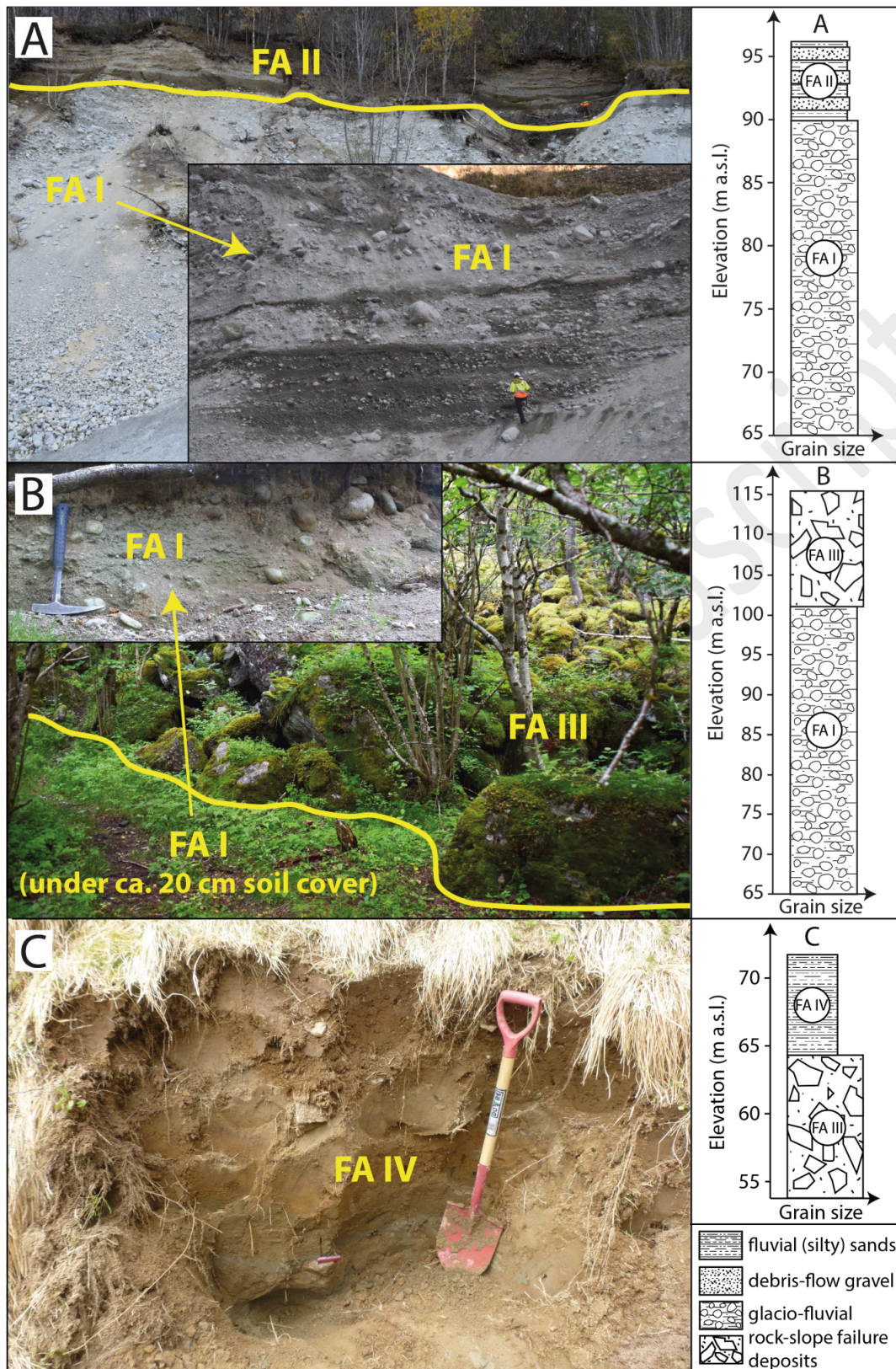
Figure 4: Impressions from the locations of the composite sediment profiles and the sediment characteristics: A) Gravel pit with ca. 35 m stratified drift (FA I) and ca. 7 m interbedded fluvial sands in angular debris-flow gravel (FA II), person is 1,70m tall; B) ca. 15 m thick chaotic boulder deposits (FA III) on top of FA I, which is only visible in small outcrops; C) silty sands with outsized cobbles on top of ca. 10m thick rock-slope failure boulders.
