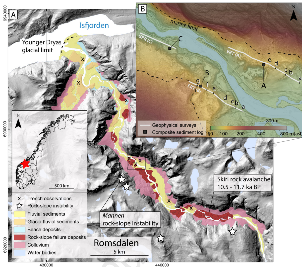
Figure 1: Overview over the study area: A) Quaternary geology of the lower and mid Romsdal Valley; B) detail of the main study site and the locations of geophysical surveys and composite sediment logs. Note the stretched colour code.
