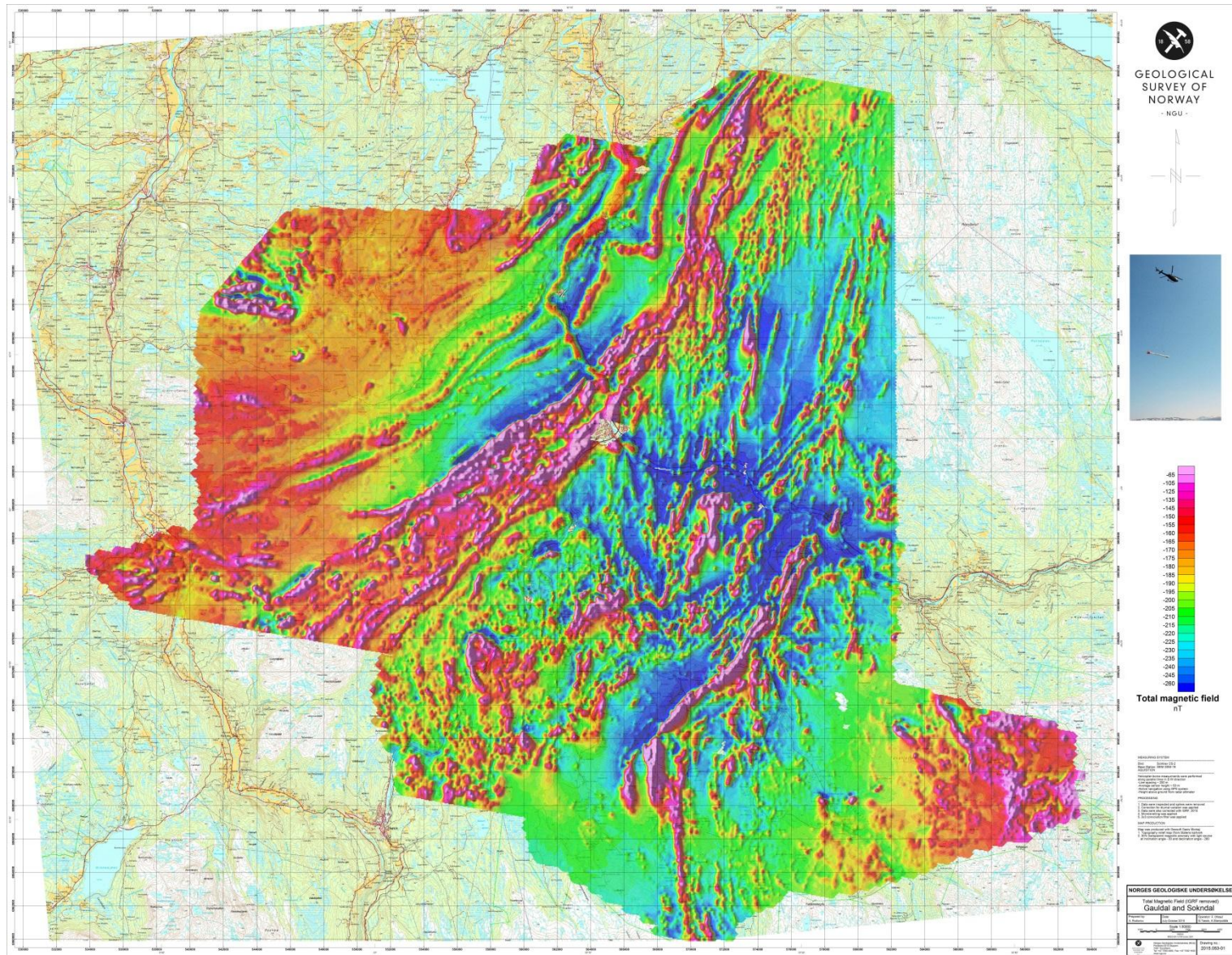
Figure 5: Total Magnetic Field
