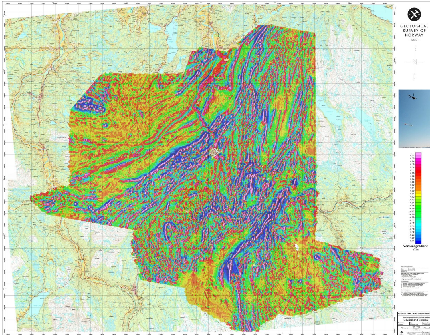
Figure 6: Magnetic Vertical Derivative
