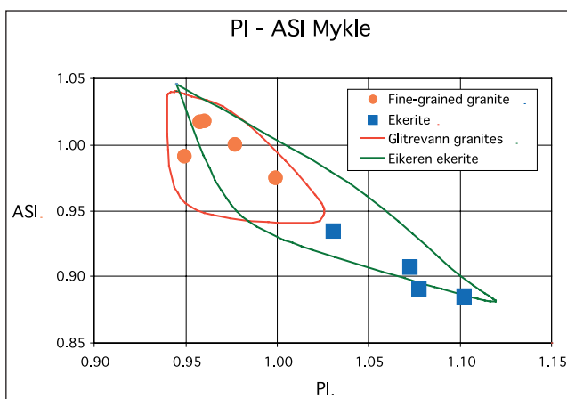
Fig. 8. PI-ASI diagram. The Alumina Saturation Index is defined as the Al_2O_3/(CaO + Na_2O + K_2O) molar ratio. The Peralkalinity Index PI is defined as the (Na_2O + K_2O)/Al_2O_3 molar ratio. The polygonal areas are the composition fields of the Glitrevann Cauldron (adapted from Jensen 1985) and the Eikeren ekerite (adapted from Neumann et al. 1990).
