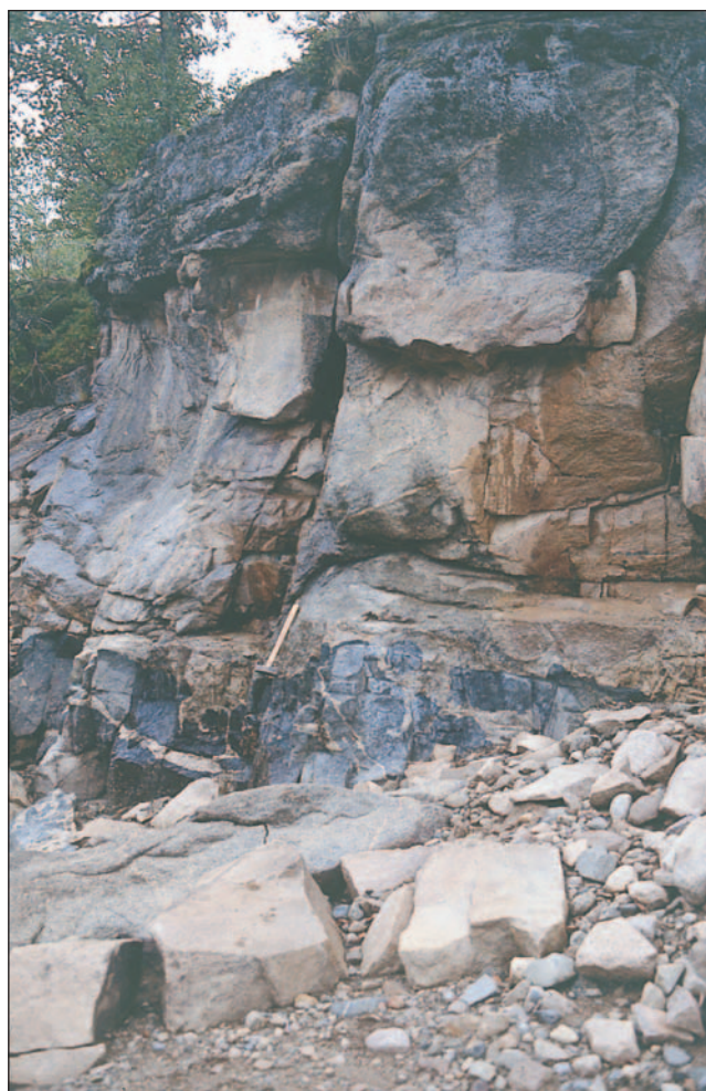
Fig. 3. Contact between larvikite (top part of the photo) and the underlying granite which, in the upper part, is devoid of mafic globules but, in the lower part, contains such globules. Southwest coast of Mykle.
