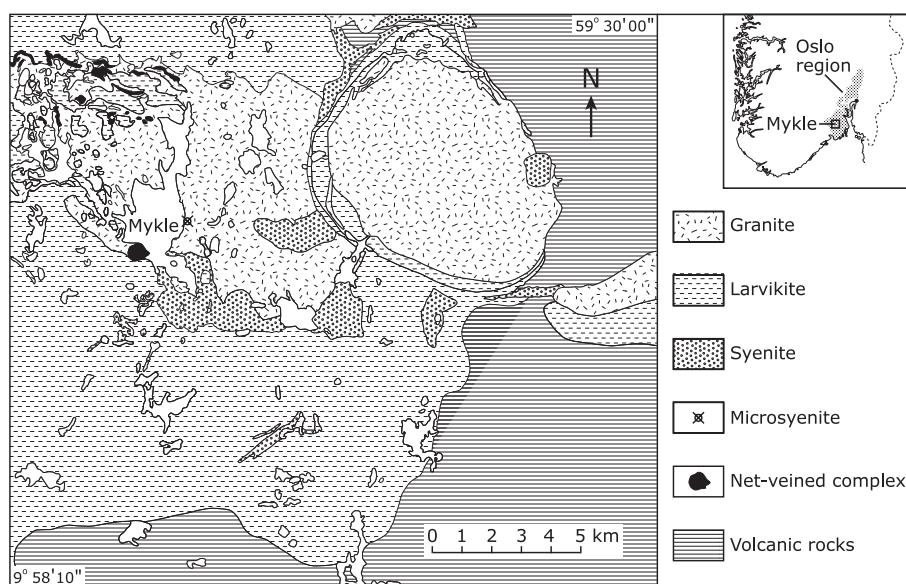
Fig. 2. Simplified geological map of the Mykle area. The contact between the fine- to medium-grained granite and the ekerite is not shown due to poor exposures in large parts of the area. The ekerite occupies the central part, and the fine- to medium-grained granite the marginal parts of the western granite massif.
