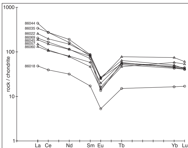
Fig. 9. Chondrite-normalised REE diagram.
