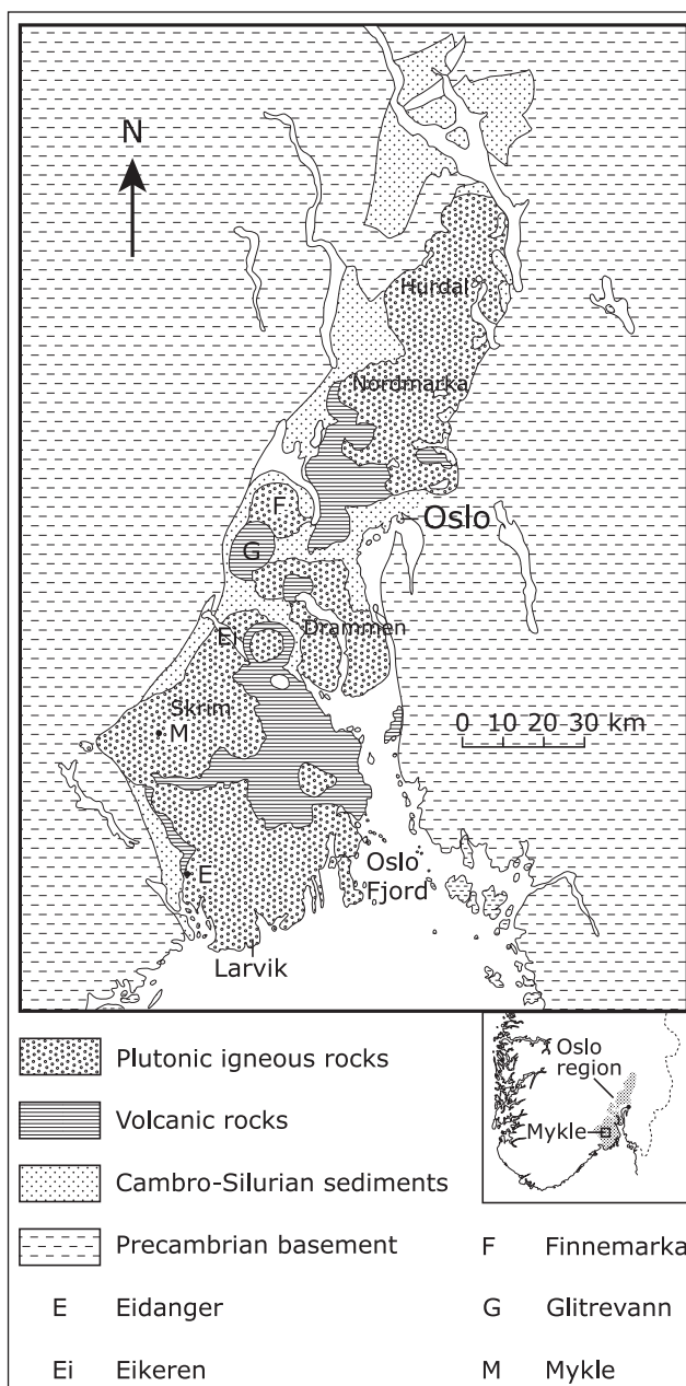
Fig. 1. Generalised geological map of the Oslo Igneous Province.
